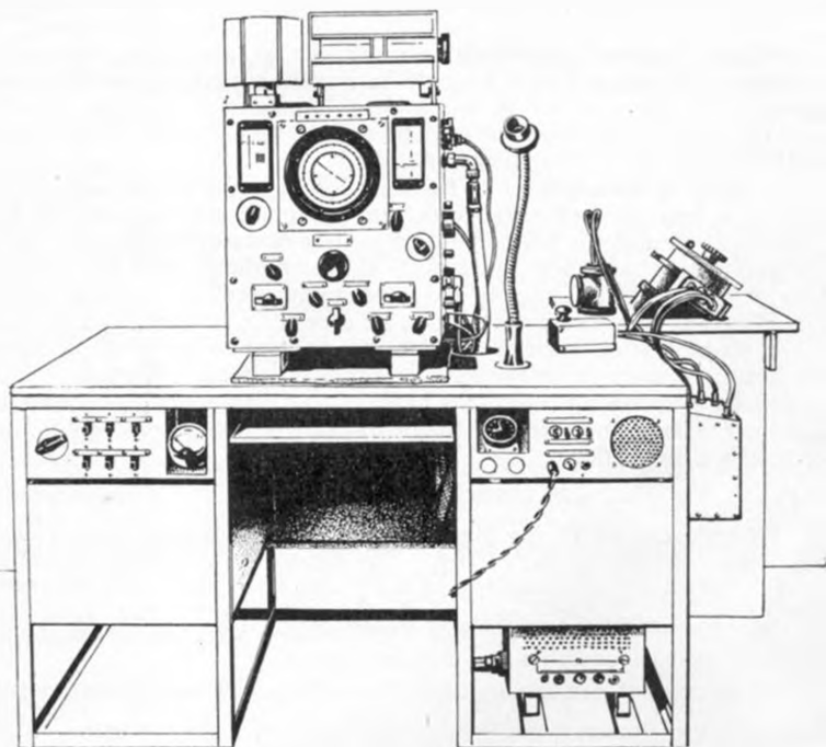
Fig. 88. D/F equipment—A.H.6
